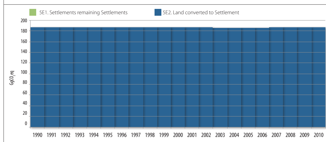
Figure 67. Settlements: GHG emission and removal trend per subcategory, 1990 - 2010 series.
