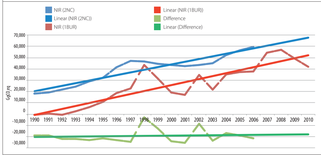
Figure 78. Chile's NIR: net GHG emission trend reported in the Second National Communication of Chile and the First Biennial Update Report, 1990 - 2010 series.
