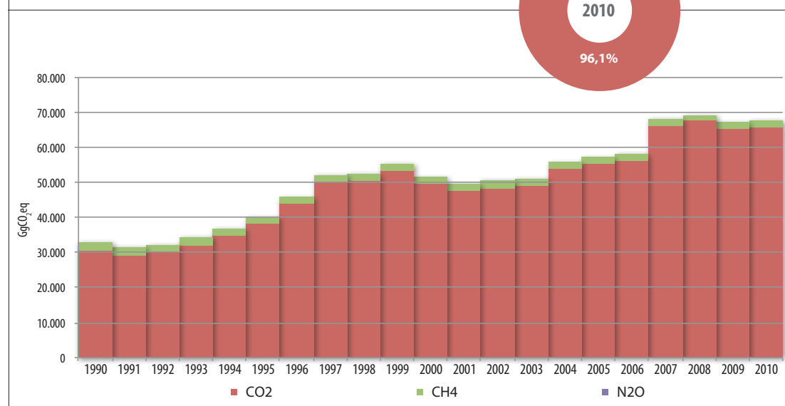
Figure 11. Energy Sector: emissions per GHG type (GgCO 2 eq), 1990 - 2010 series .
